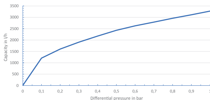
Capacity Dirt Separator 22C
